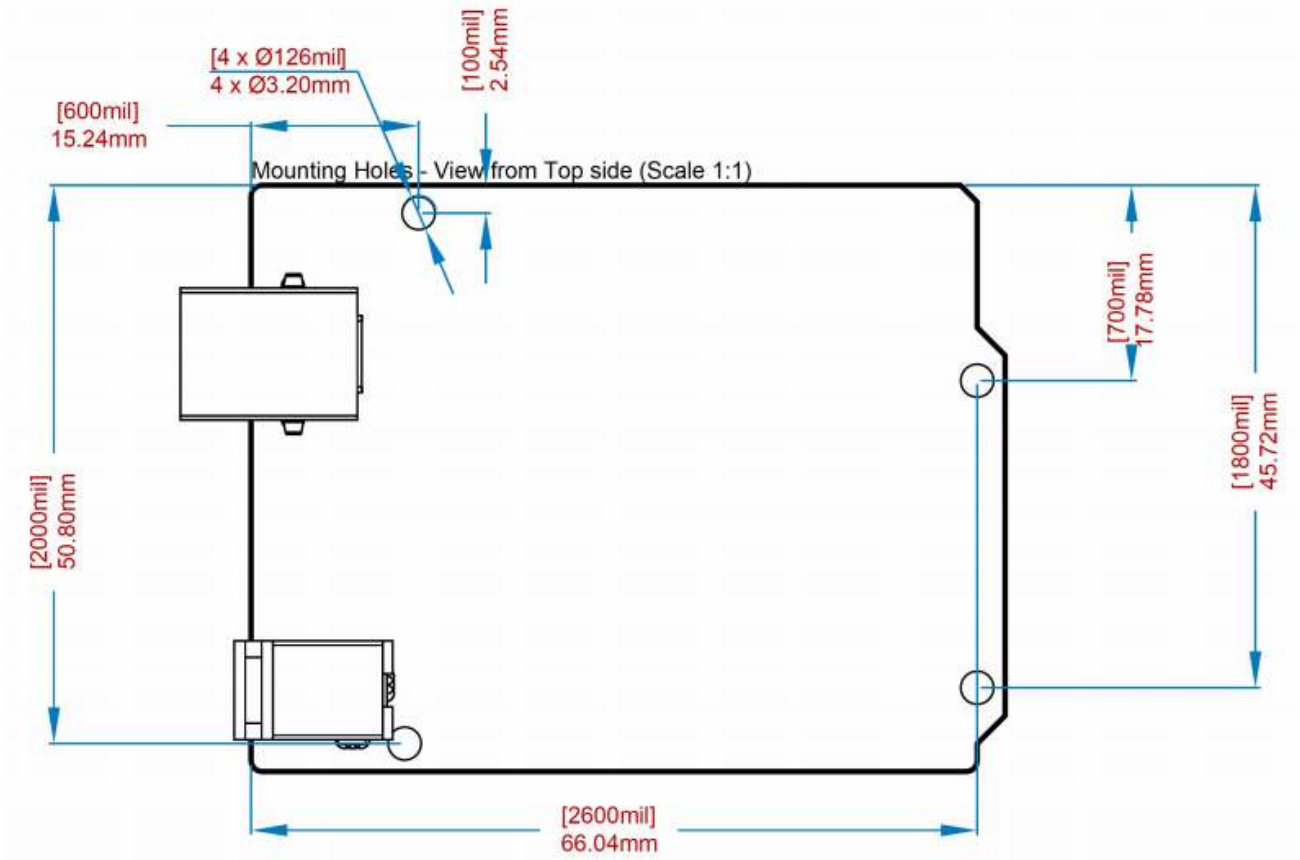
Board outline
